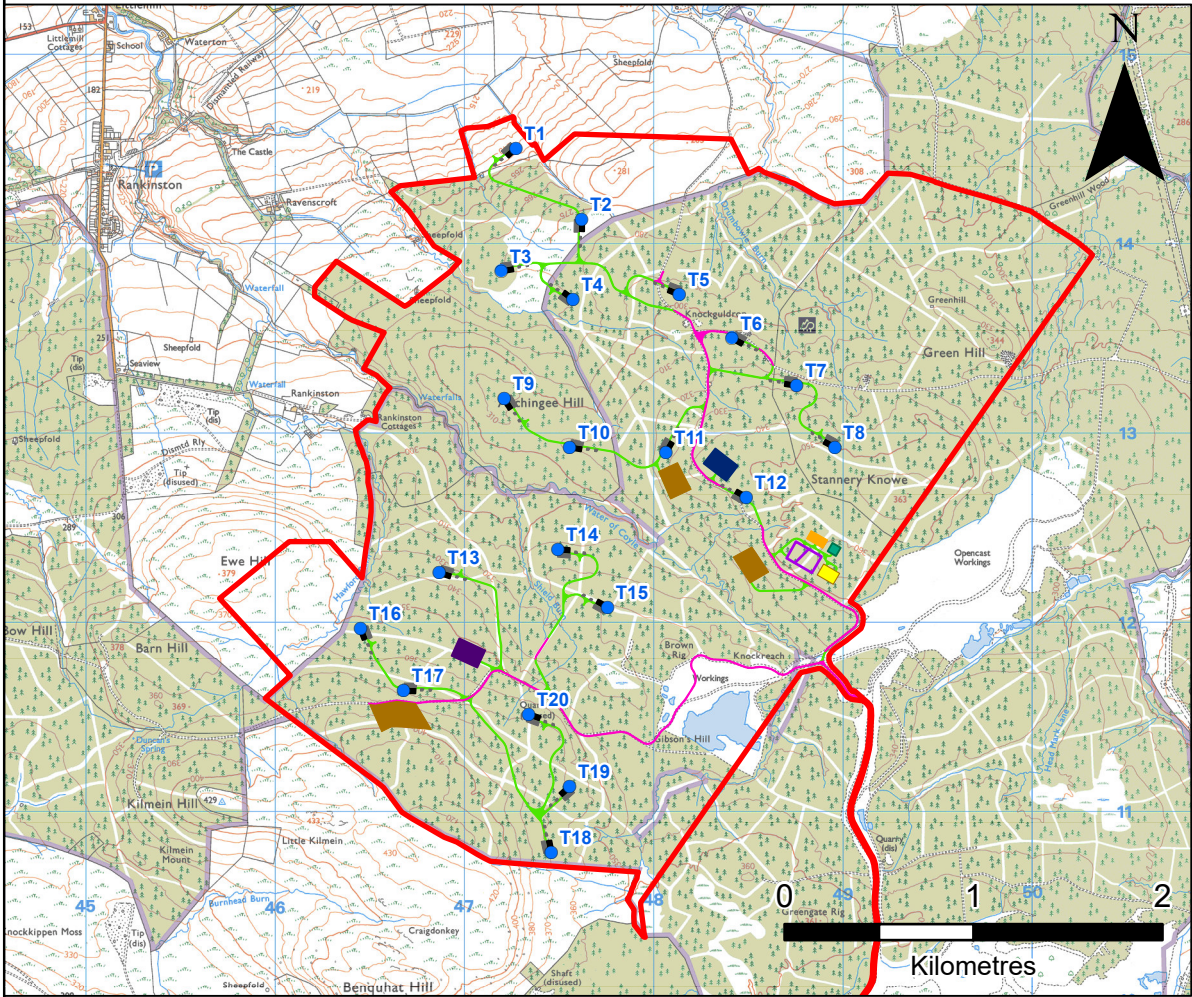
DESIGN FREEZE LAYOUT (MAY 2025)
